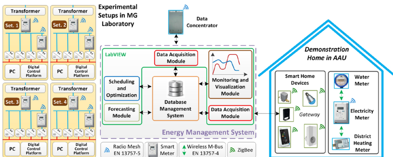
Fig. 1. Advanced Smart Metering Infrastructure and Energy Management System in Microgrid Research Laboratory at Aalborg University.
